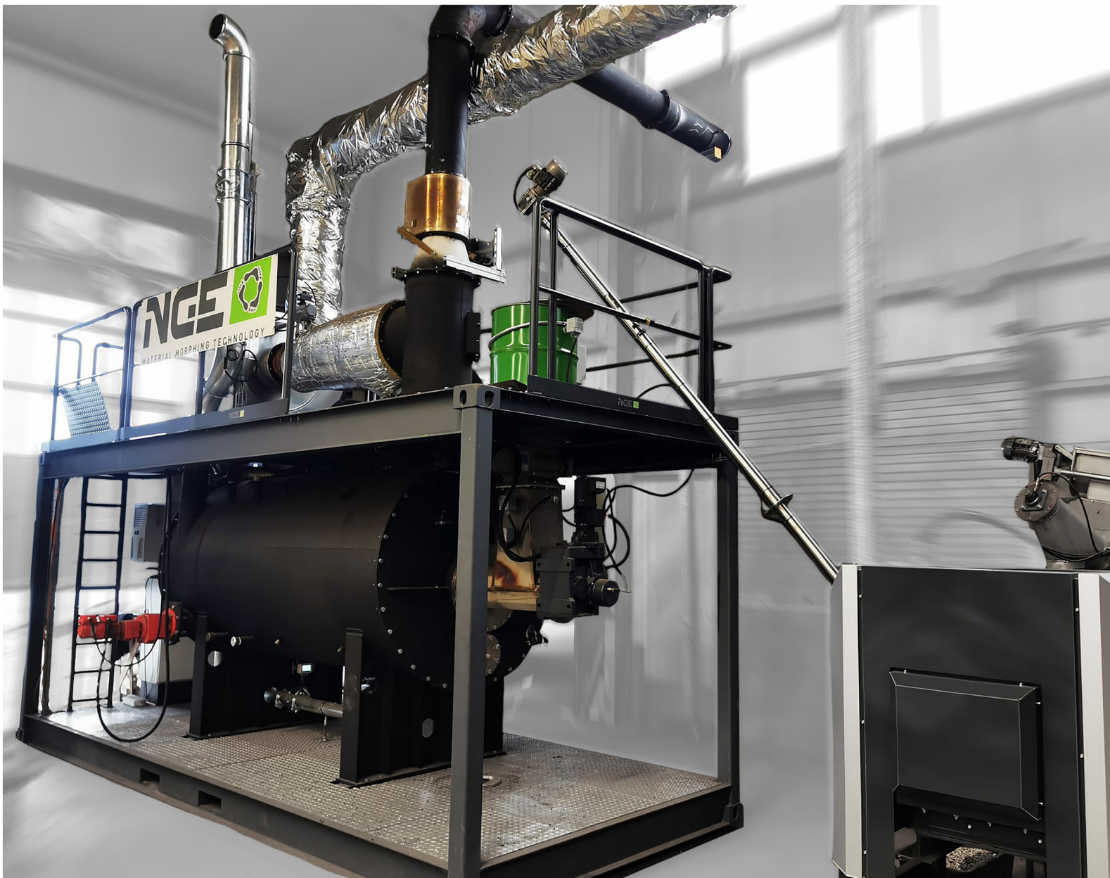
Pilot plant PyroDry ® 3000
